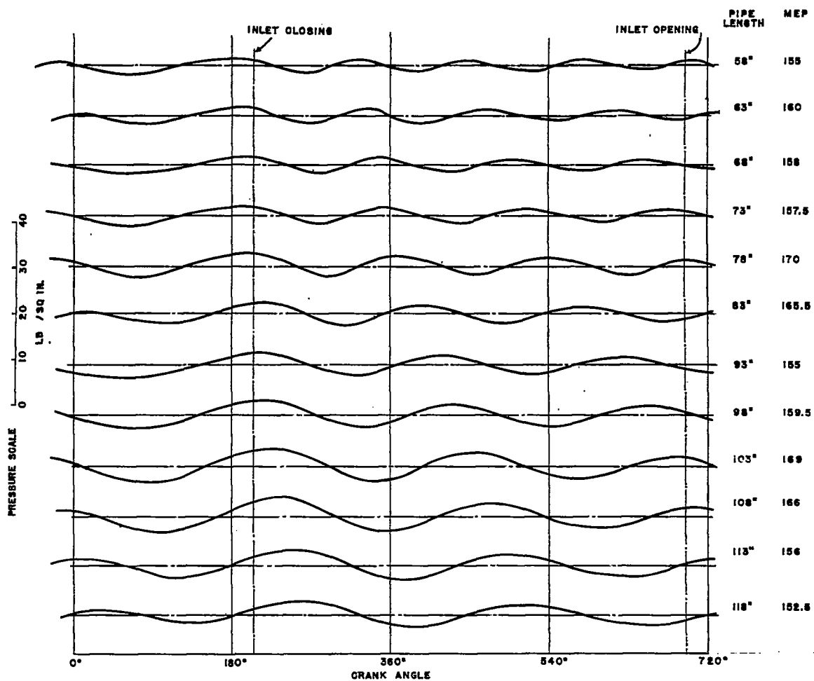
PRESSURE IN INLET PIPE FOR VARIOUS PIPE LENGTHS AT CONSTANT INLET CLOSING RPM 1220 PIPE DIAMETER 2.56 IN.
