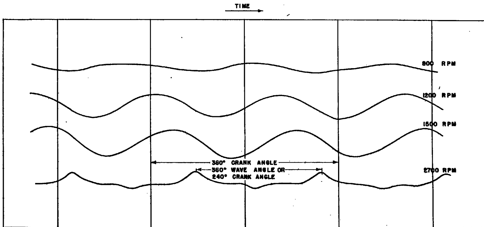
PRESSURE CURVES AT VARIOUS R P M 72 INCH PIPE
