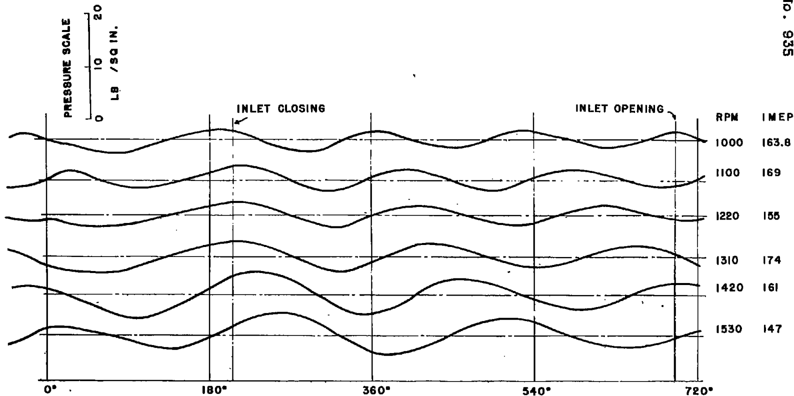
PRESSURE IN PIPE AT DIFFERENT RPM PIPE LENGTH 93 IN. DIAMETER 2.56 IN.
