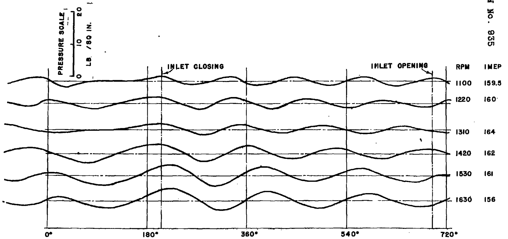
PRESSURE IN PIPE AT DIFFERENT RPM PIPE LENGTH 63 IN. DIAMETER 2.56 IN.
