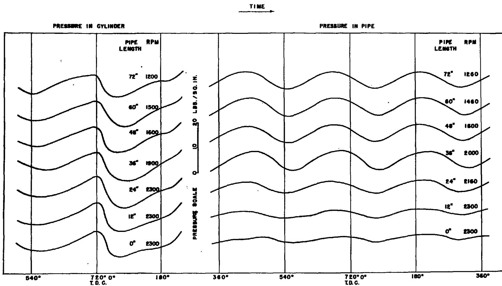
PRESSURE CURVES FOR BEST VOLUMETRIC EFFICIENCY
