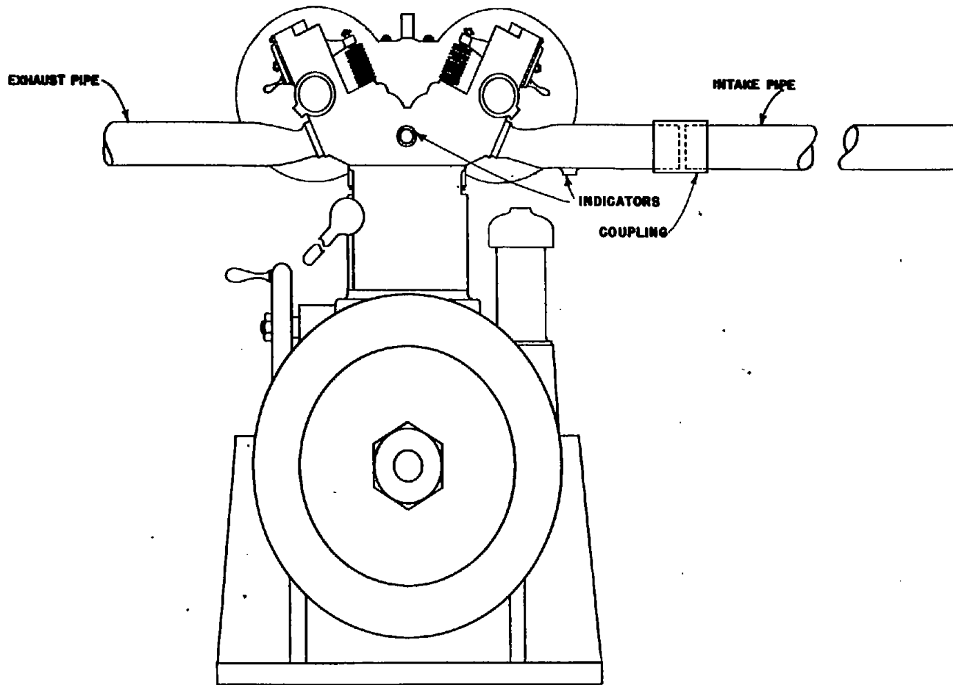
NACA UNIVERSAL TEST ENGINE Figure 2.
