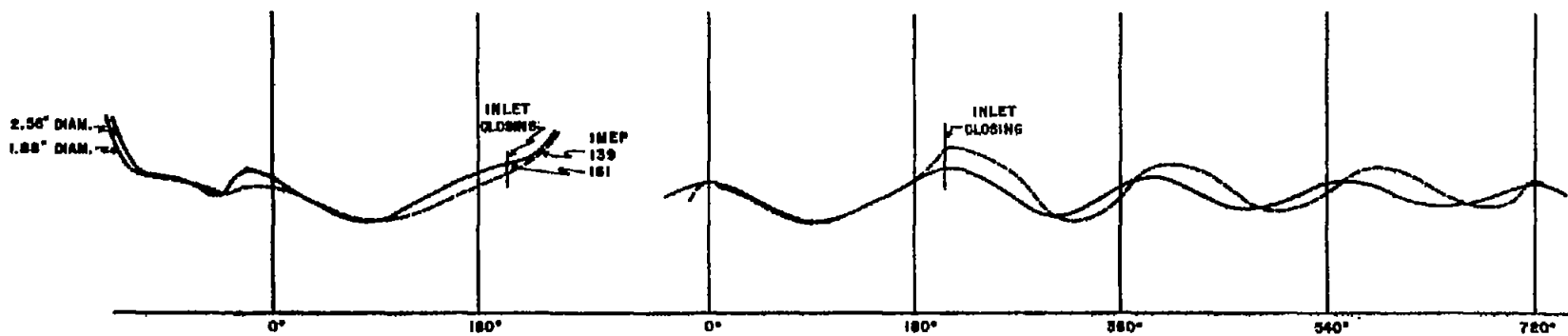
PRESSURE WAVES IN PIPE AND CYLINDER FOR 2.56" AND 1.88" DIAMETER PIPE RPM 1600 PIPE LENGTH 59 IN.
